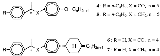
Fig. 2. The structural formula of new chiral dopants.
